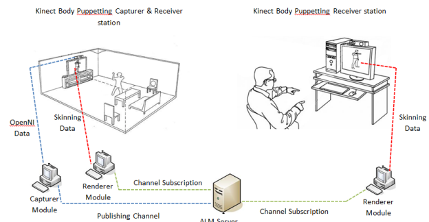
Figure 9: Kinect Body-Puppeting module architecture
