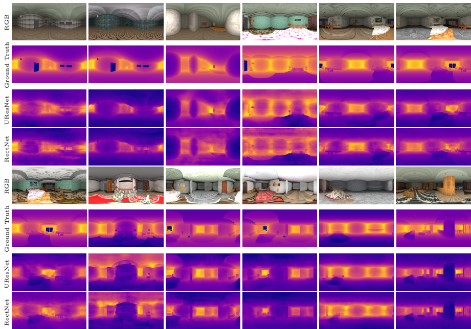
Fig. 4: Qualitative results of our models on our SceneNet [4] renders. (best viewed in color – paper – and zoomed in – screen)
