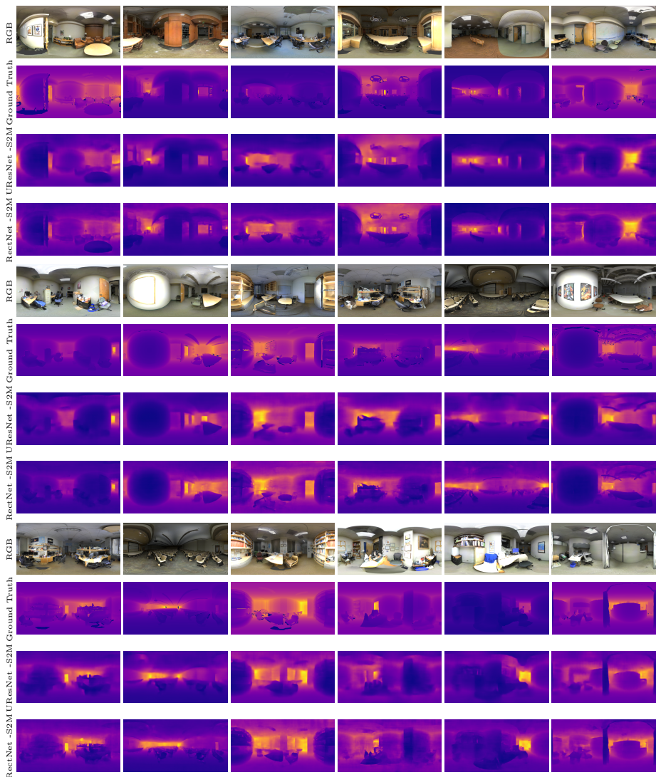
Fig. 6: Qualitative results of UResNet-S2M and RectNet-S2M, which are trained on SunCG [3] and fine tuned on Matterport3D [1], on the left out dataset used for validation, Stanford2D3D [2]. (best viewed in color – paper – and zoomed in – screen)
