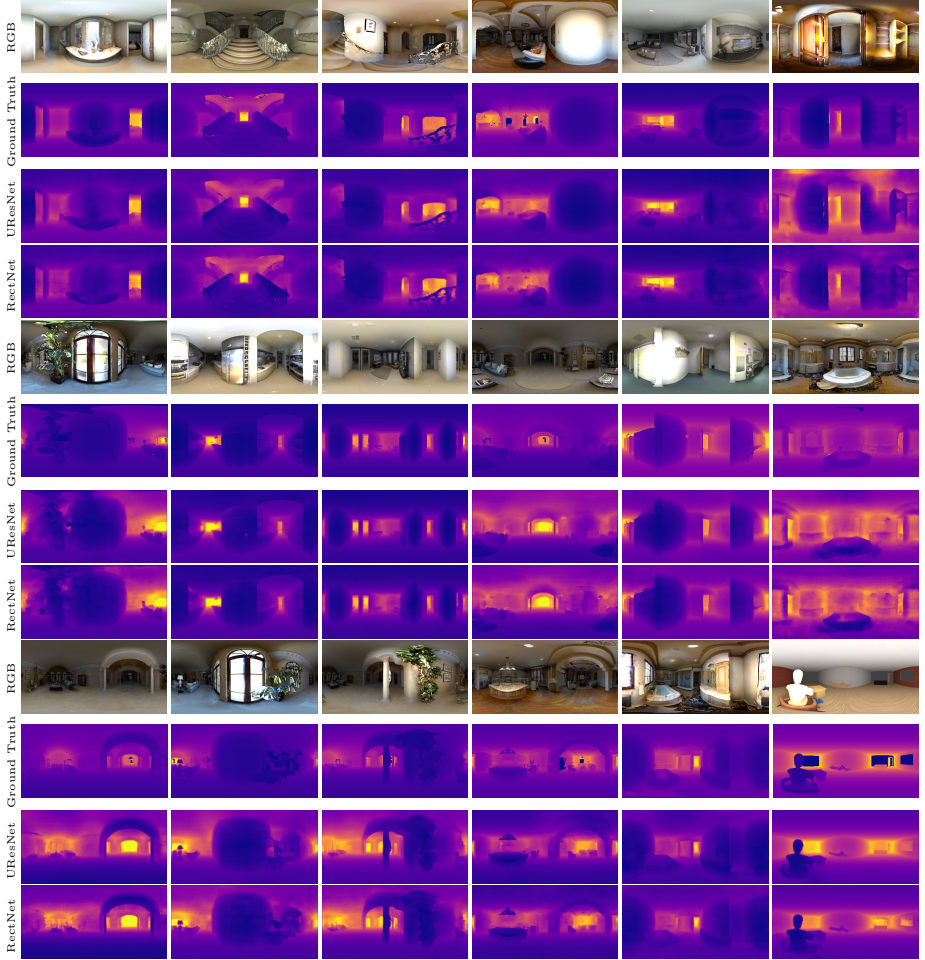
Fig. 3: Additional qualitative results of the UResNet and RectNet models are presented on our test set. (best viewed in color – paper – and zoomed in – screen)
