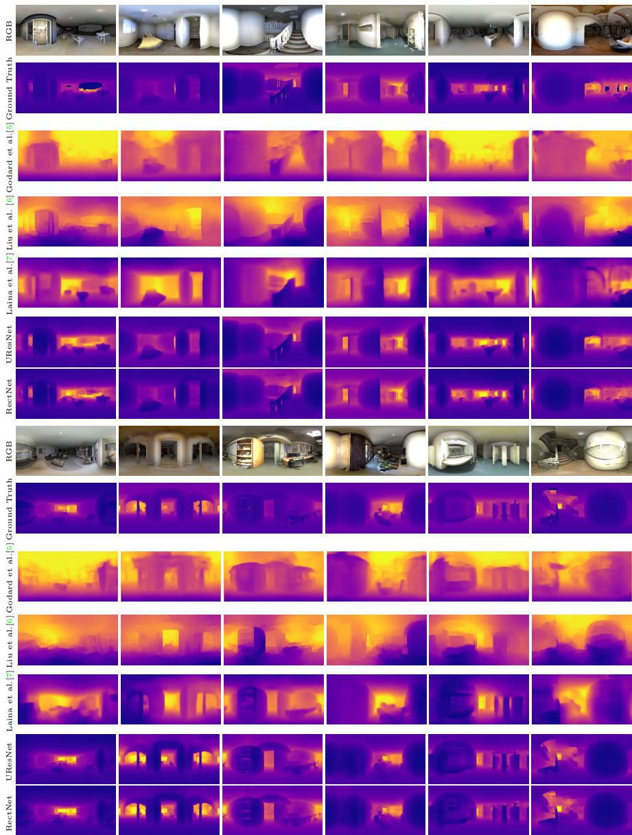
Fig. 2: Qualitative comparisons against monocular models applied directly on the equirectangular image. The original rendered color image along with its corresponding ground truth are presented. In addition, we offer results of Godard et al. [5], Liu et al. [6], Laina et al. [7], as well as our model predictions, the URResNet and RectNet networks. (best viewed in color – paper – and zoomed in – screen)
