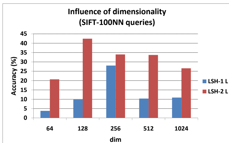
Fig. 4 LSH' retrieval accuracy versus dimensionality for 100-NN queries in SIFT datasets.
